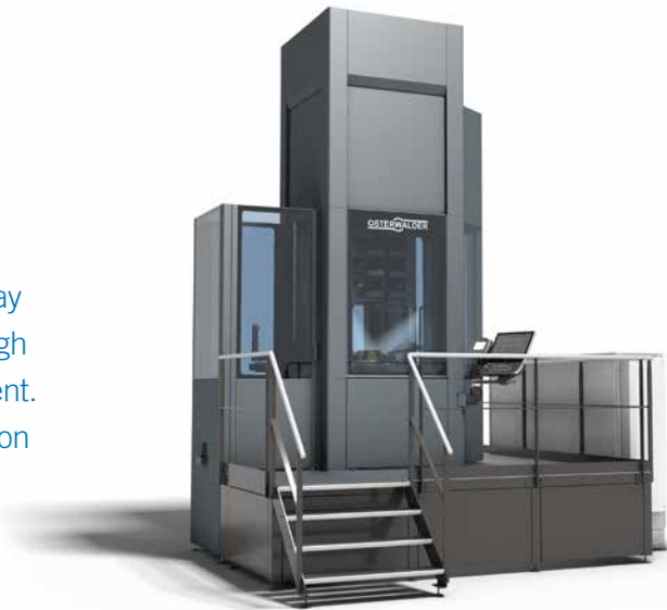
Osterwalder – World's first electric multi-level powder press for high pressing forces of up to 2,000 kN
