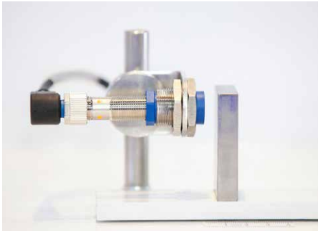
Proximity sensor with safety function for construction machinery
