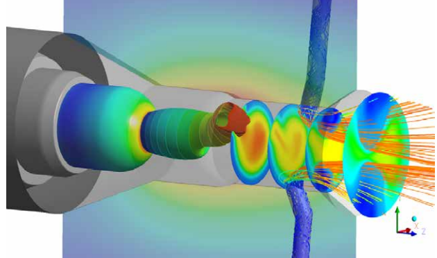
Multiphysics modelling and simulation of simultaneous processes in a plasma spray pistol
