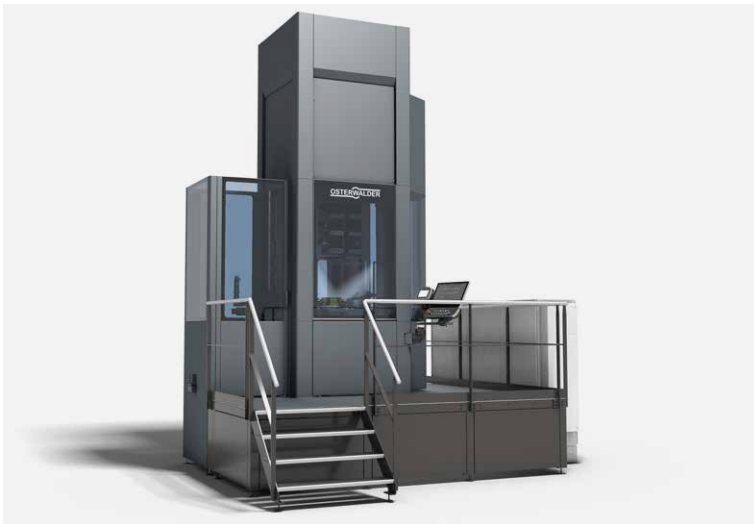
Development of a resource-efficient powder press: thanks to intelligent servo-electric drives, electricity consumption can be reduced by over 80% and water consumption by 75%. The press also requires less servicing and is cheaper to run.
